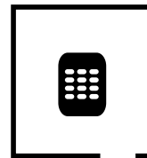
Code
